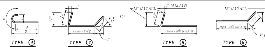
Reinforcement Details
